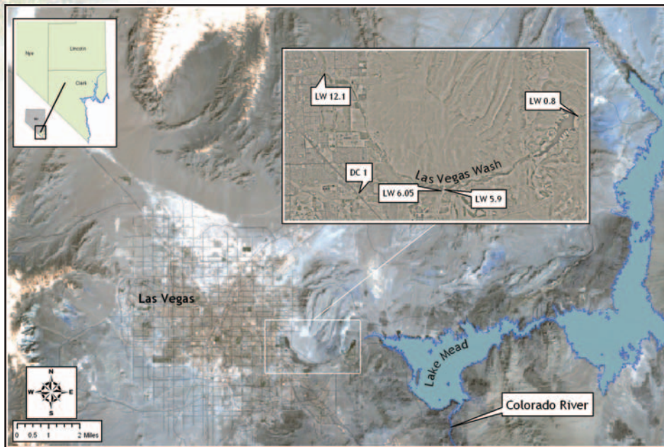
Sites selected for near-real-time water quality monitoring in the Las Vegas Wash.
